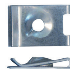
Plate nut, speednut M8
